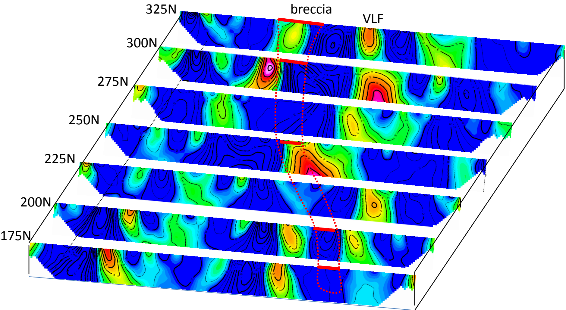
South Breccia Fence Diagram VLF-EM Pseudo-sections
